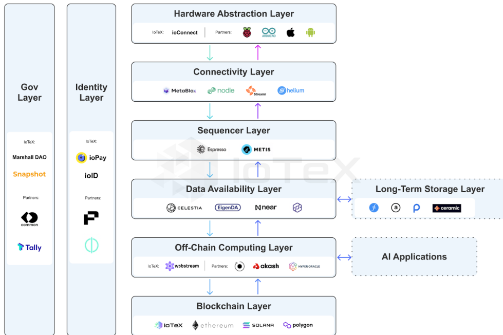
Figure 2.2: The DePIN Infrastructure Modules (DIMs)
