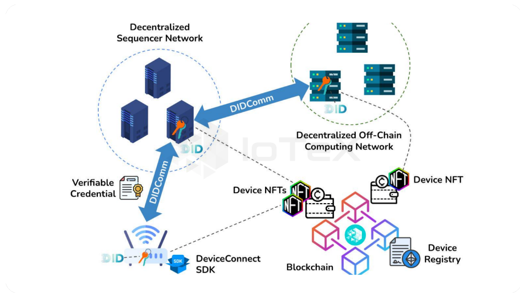
Figure 5.2: An Overview of the ioID Identity System
