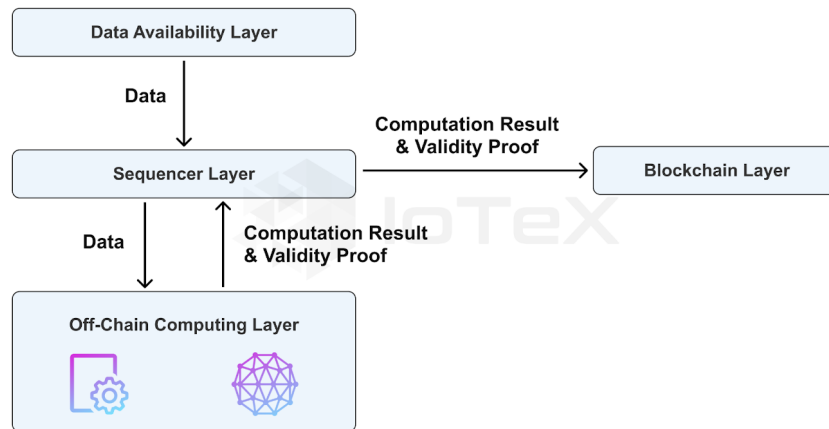
Figure 4.6: The High-Level Workflow of the Off-Chain Computing Layer
