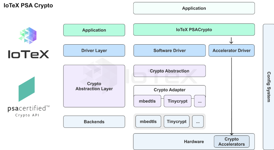
Figure 6.3: The Usage of IoTeX’s PSACrypto Library in DePIN Devices
