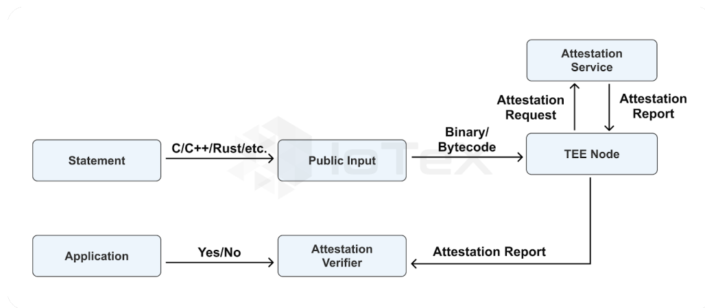
Figure 4.4: The System Architecture of a TEE-Based Application
