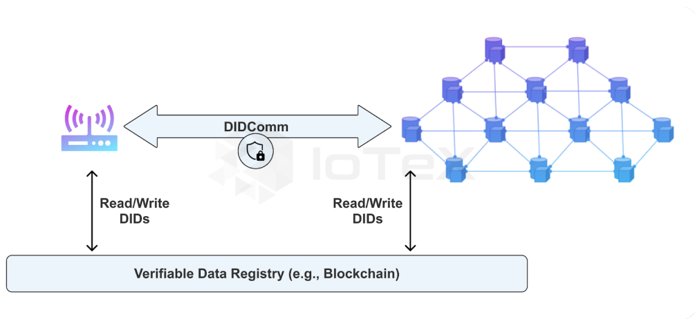
Figure 6.4: SSI-Based Communication in a Decentralized Setting
