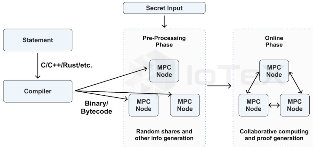
Figure 4.5: The System Architecture of a SMPC-Based Application
