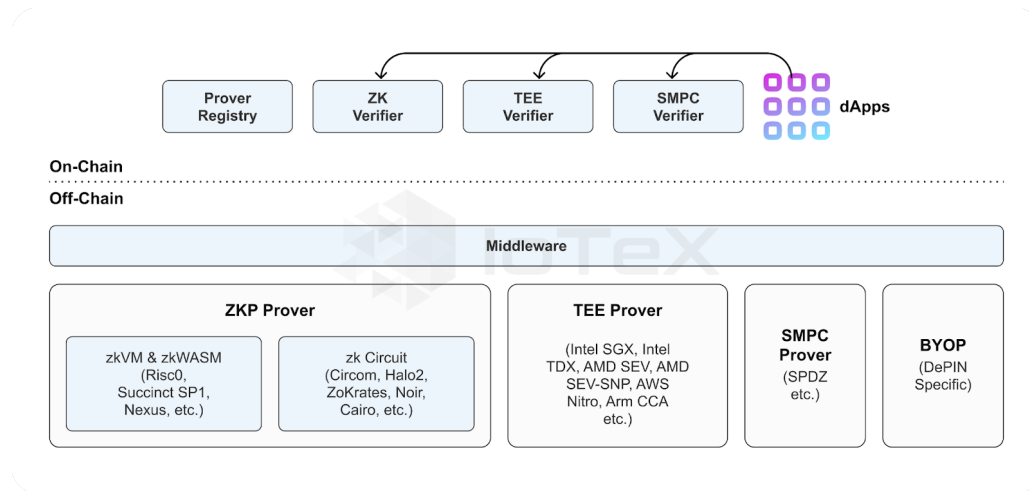
Figure 4.1: W3bstream in a Nutshell
