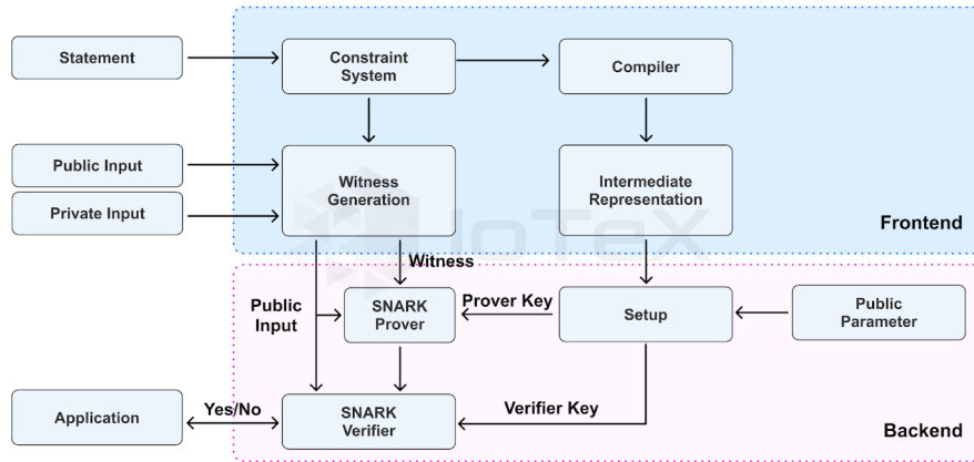
Figure 4.3: The System Architecture of a SNARK-Based Application Built upon a Customized Circuit
