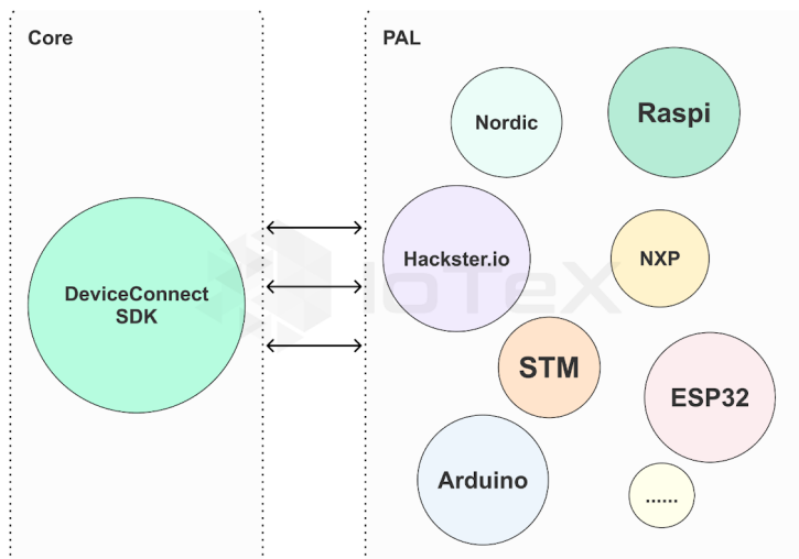
Figure 6.6: The Layered Architecture in the ioConnect SDK
