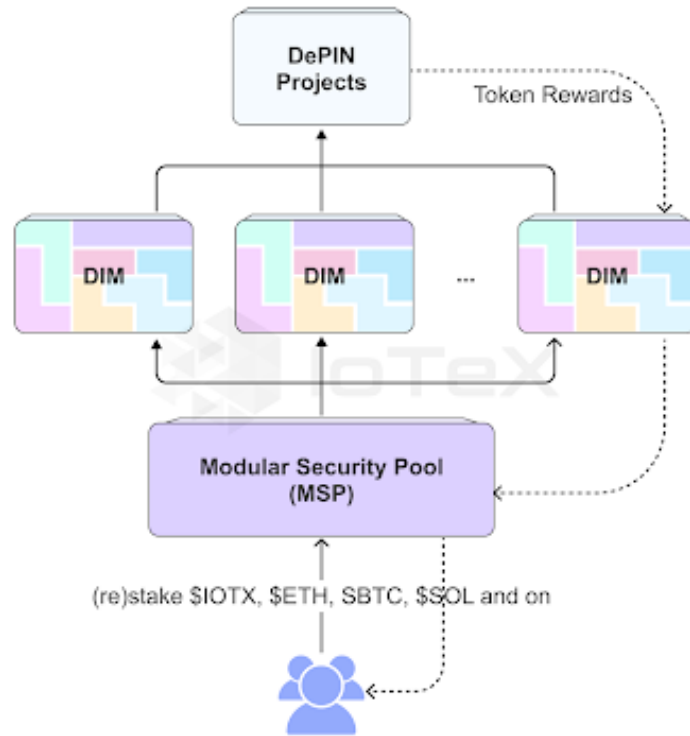
Figure 3.1: The Architecture of the Modular Security Pool (MSP)
